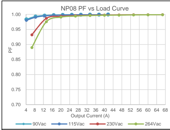
Figure 13: NP08W1-1MW0(8)-00-18P-A-0 PF vs Load Curve
