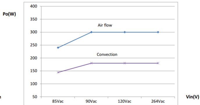
SLB350S12K
