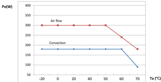
SLB350S12K
