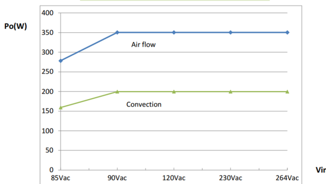
SLB350S24K/SLB350S48K/SLB350S56K
