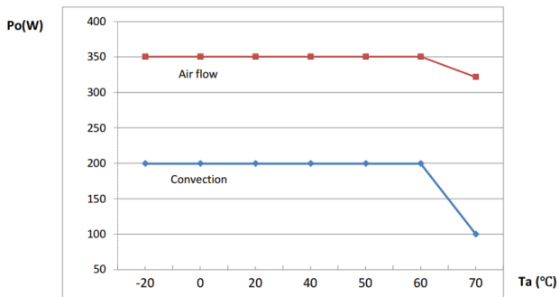
SLB350S24K/SLB350S48K/SLB350S56K
