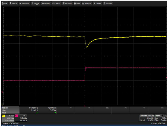
Figure 79: LCM30007-T Transient Response - Vo Deviation 50% to 100% load change 1A/uS slew rate Vin = 230Vac Ch 1: Vo Ch 2: Io
