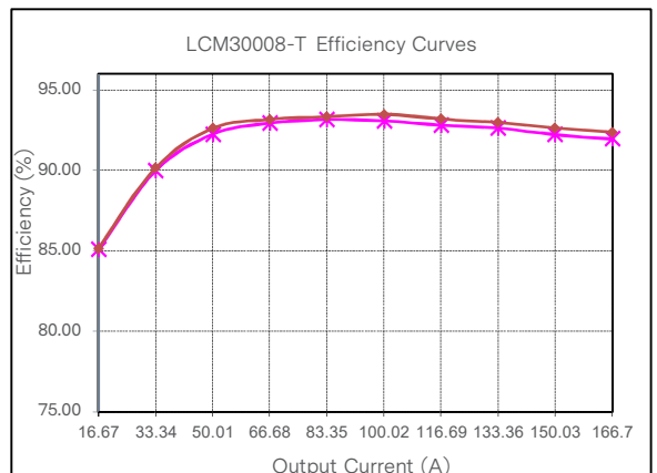
Figure 26: LCM30008-T Efficiency Curve @ 25°C Loading: Io_main = 10%Io_max increment to 166.7A, Isb = 0A
