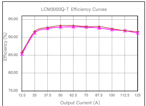
Figure 40: LCM3000Q-T Efficiency Curve @ 25°C Loading: Io_main = 10%Io_max increment to 125A, Isb = 0A
