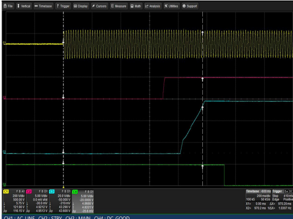
Figure 57: LCM3000W-T Turn-on delay via AC mains Vin = 90Vac Load: Io = 31.25A (48V), Isb = 2A Ch 1: Vin Ch 2: Vsb Ch 3: Vo Ch 4: G_DCOK_C
