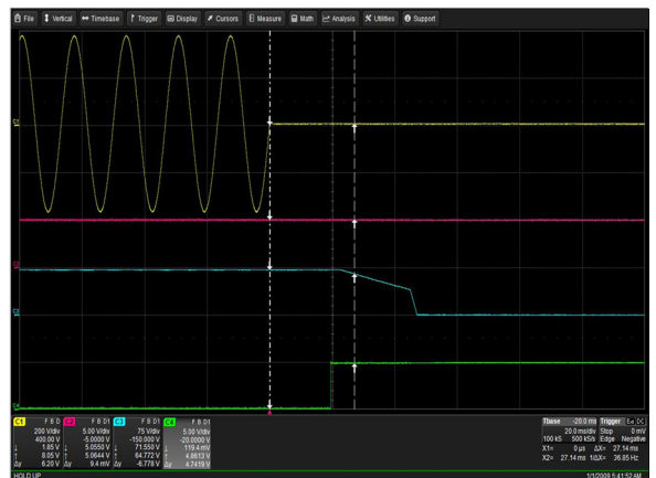
Figure 76: LCM30007-T Hold-up Time Vin = 264Vac Load: lo = 41.7A (72V), Isb = 2A Ch 1: Vin Ch 2: Vsb Ch 3: Vo Ch 4: G_DCOK_C
