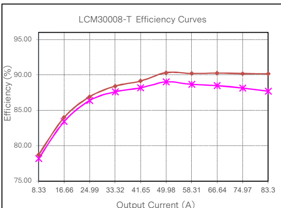
Figure 25: LCM30008-T Efficiency Curve @ 25°C Loading: Io_main = 10%Io_max increment to 83.3A, Isb = 0A
