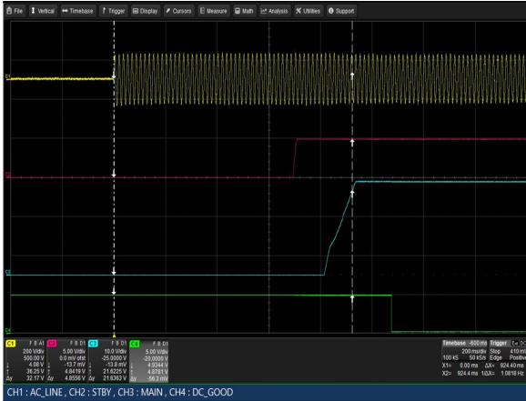
Figure 29: LCM3000Q-T Turn-on delay via AC mains Vin = 90Vac Load: Io = 62.5A (24V), Isb = 2A Ch 1: Vin Ch 2: Vsb Ch 3: Vo Ch 4: G_DCOK_C
