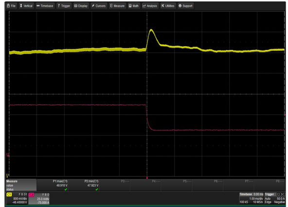
Figure 66: LCM3000W-T Transient Response - Vo Deviation 100% to 50% load change 1A/uS slew rate Vin = 230Vac Ch 1: Vo Ch 2: Io
