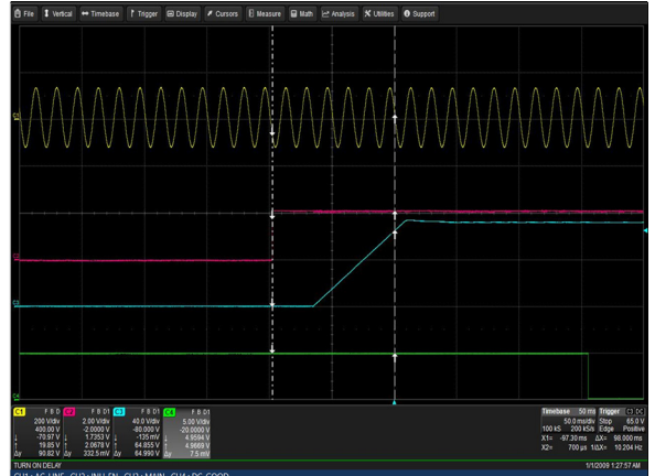
Figure 72: LCM30007-T Turn-on delay via INH_EN Vin = 90Vac Load: lo = 20.8A (72V), Isb = 2A Ch 1: Vin Ch 2: INH_EN Ch 3: Vo Ch 4: G_DCOK_C
