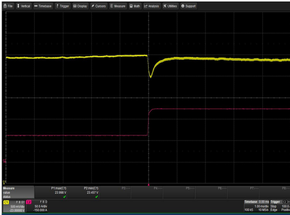
Figure 37: LCM3000Q-T Transient Response - Vo Deviation 50% to 100% load change 1A/uS slew rate Vin = 230Vac Ch 1: Vo Ch 2: Io
