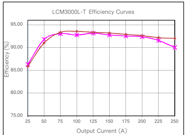
Figure 12: LCM3000L-T Efficiency Curve @ 25°C Loading: Io_main = 10%Io_max increment to 250A, Isb = 0A
