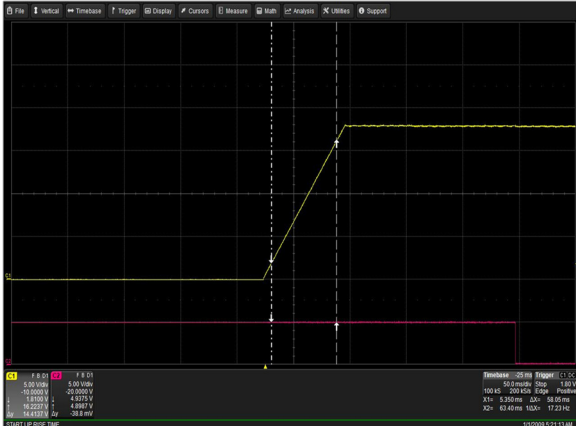
Figure 21: LCM30008-T Output Voltage Startup Vin = 264Vac Load: Io = 166.7A (18V), Isb = 2A Ch 1: Vo Ch 2: G_DCOK_C
