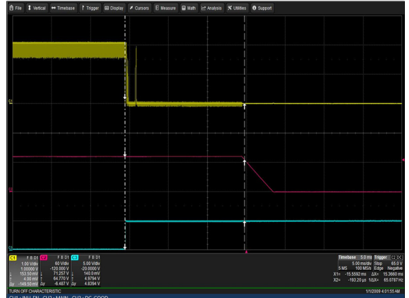
Figure 78: LCM30007-T Turn Off Characteristic via INH_EN Vin = 264Vac Load: Io = 41.7A (72V), Isb = 2A Ch 1: INH_EN Ch 2: Vo Ch 3: G_DCOK_C
