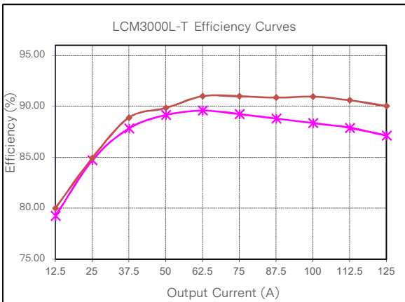
Figure 11: LCM3000L-T Efficiency Curve @ 25°C Loading: Io_main = 10%Io_max increment to 125A, Isb = 0A
