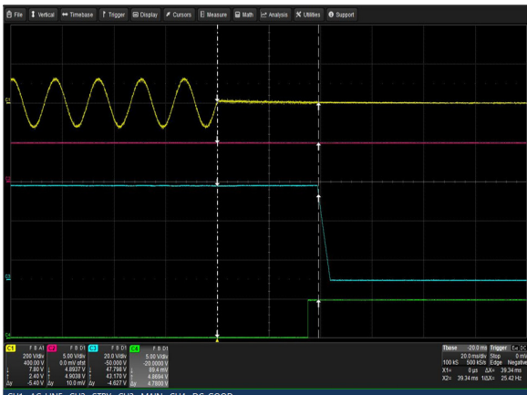
Figure 61: LCM3000W-T Hold-up Time Vin = 90Vac Load: Io = 31.25A (48V), Isb = 2A Ch 1: Vin Ch 2: Vsb Ch 3: Vo Ch 4: G_DCOK_C
