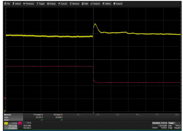
Figure 38: LCM3000Q-T Transient Response - Vo Deviation 100% to 50% load change 1A/uS slew rate Vin = 230Vac Ch 1: Vo Ch 2: Io
