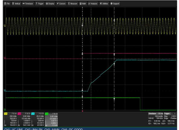
Figure 58: LCM3000W-T Turn-on delay via INH_EN Vin = 90Vac Load: Io = 31.25A (48V), Isb = 2A Ch 1: Vin Ch 2: INH_EN Ch 3: Vo Ch 4: G_DCOK_C
