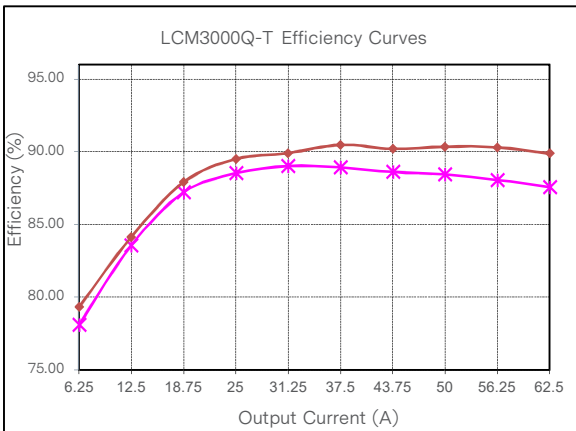
Figure 39: LCM3000Q-T Efficiency Curve @ 25°C Loading: Io_main = 10%Io_max increment to 62.5A, Isb = 0A
