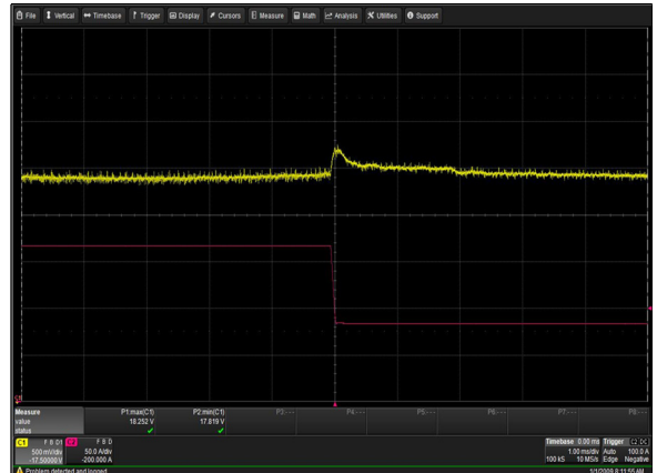
Figure 24: LCM30008-T Transient Response - Vo Deviation 100% to 50% load change 1A/uS slew rate Vin = 230Vac Ch 1: Vo Ch 2: Io
