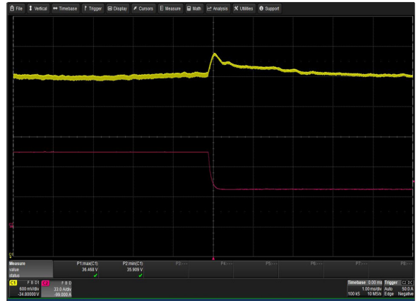
Figure 52: LCM3000U-T Transient Response - Vo Deviation 100% to 50% load change 1A/uS slew rate Vin = 230Vac Ch 1: Vo Ch 2: Io
