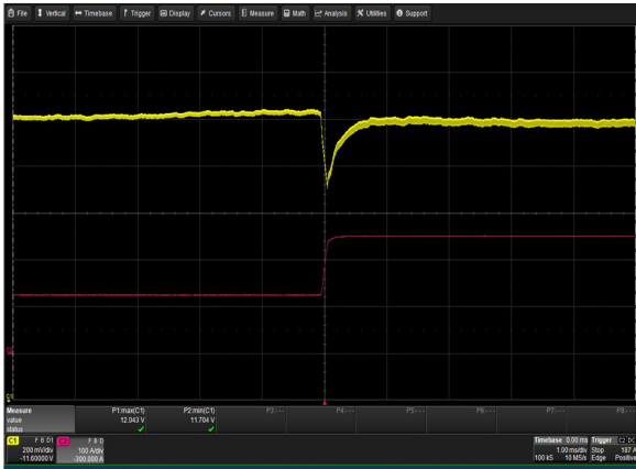
Figure 9: LCM3000L-T Transient Response - Vo Deviation 50% to 100% load change 1A/uS slew rate Vin = 230Vac Ch 1: Vo Ch 2: Io
