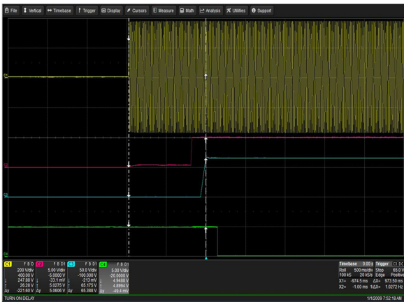
Figure 73: LCM30007-T Turn-on delay via AC mains Vin = 264Vac Load: lo = 41.7A (72V), Isb = 2A Ch 1: Vin Ch 2: Vsb Ch 3: Vo Ch 4: G_DCOK_C
