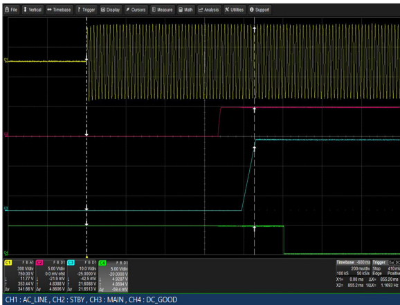
Figure 31: LCM3000Q-T Turn-on delay via AC mains Vin = 264Vac Load: Io = 125A (24V), Isb = 2A Ch 1: Vin Ch 2: Vsb Ch 3: Vo Ch 4: G_DCOK_C
