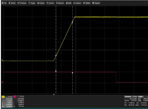
Figure 7: LCM3000L-T Output Voltage Startup Vin = 264Vac Load: Io = 125A (12V), Isb = 2A Ch 1: Vo Ch 2: G_DCOCK_C
