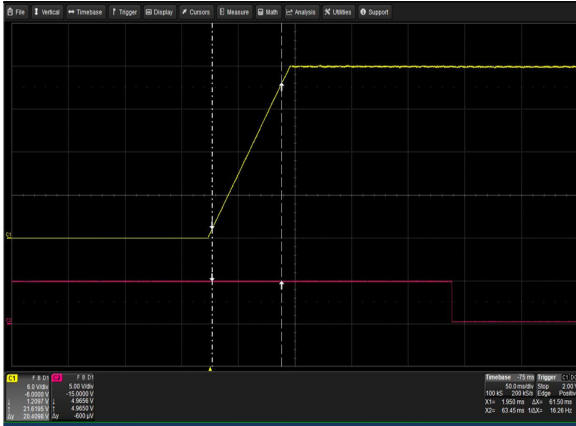
Figure 35: LCM3000Q-T Output Voltage Startup Vin = 264Vac Load: Io = 125A (24V), Isb = 2A Ch 1: Vo Ch 2: G_DCOK_C
