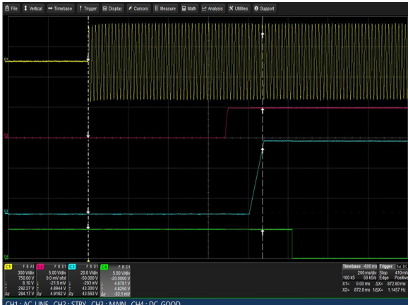
Figure 59: LCM3000W-T Turn-on delay via AC mains Vin = 264Vac Load: Io = 62.5A (48V), Isb = 2A Ch 1: Vin Ch 2: Vsb Ch 3: Vo Ch 4: G_DCOK_C
