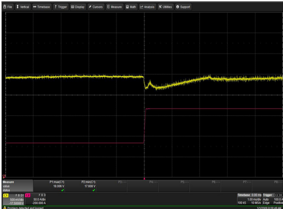
Figure 23: LCM30008-T Transient Response - Vo Deviation 50% to 100% load change 1A/uS slew rate Vin = 230Vac Ch 1: Vo Ch 2: Io
