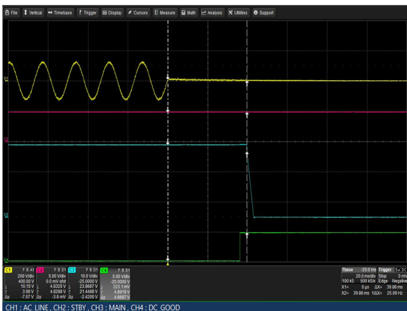
Figure 33: LCM3000Q-T Hold-up Time Vin = 90Vac Load: Io = 62.5A (24V), Isb = 2A Ch 1: Vin Ch 2: Vsb Ch 3: Vo Ch 4: G_DCOK_C
