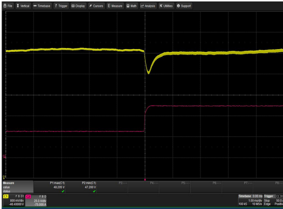
Figure 65: LCM3000W-T Transient Response - Vo Deviation 50% to 100% load change 1A/uS slew rate Vin = 230Vac Ch 1: Vo Ch 2: Io
