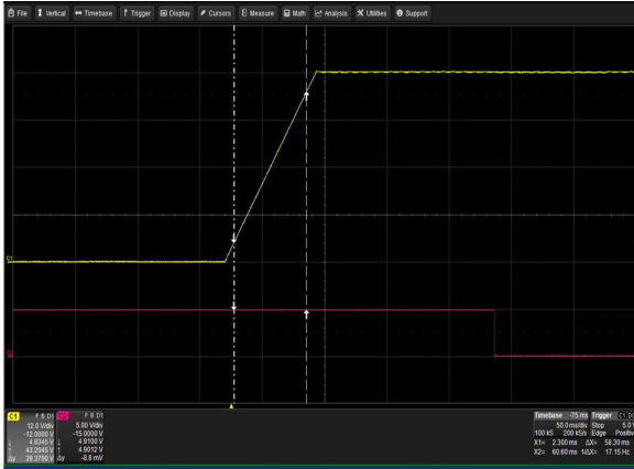
Figure 63: LCM3000W-T Output Voltage Startup Vin = 264Vac Load: Io = 62.5A (48V), Isb = 2A Ch 1: Vo Ch 2: G_DCOK_C
