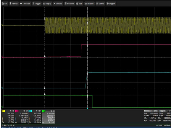
Figure 71: LCM30007-T Turn-on delay via AC mains Vin = 90Vac Load: lo = 20.8A (72V), Isb = 2A Ch 1: Vin Ch 2: Vsb Ch 3: Vo Ch 4: G_DCOK_C
