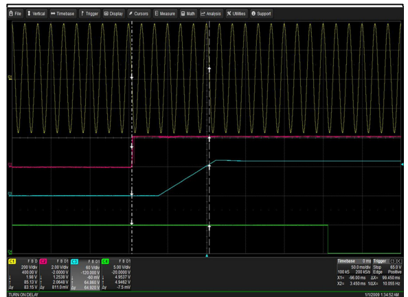
Figure 74: LCM30007-T Turn-on delay via INH_EN Vin = 264Vac Load: lo = 41.7A (72V), Isb = 2A Ch 1: Vin Ch 2: INH_EN Ch 3: Vo Ch 4: G_DCOK_C
