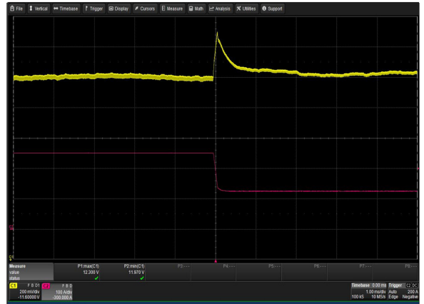
Figure 10: LCM3000L-T Transient Response - Vo Deviation 100% to 50% load change 1A/uS slew rate Vin = 230Vac Ch 1: Vo Ch 2: Io
