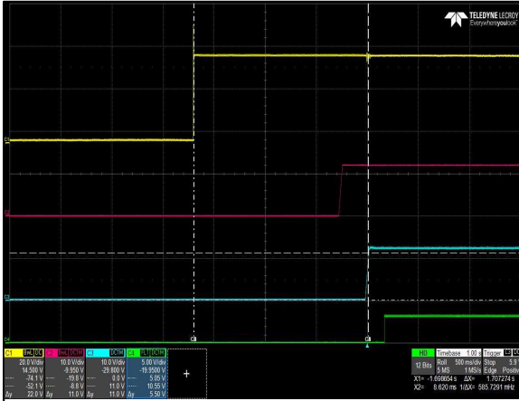
Figure 1: CSU2000ADC-3-100 Turn-On Delay via DC input Vin = -40Vdc Load: I_O = 163.9A I_{SB} = 3.5A Ch 1: V_{IN} Ch 2: V_{SB} Ch 3: V_O Ch 4: PWOK
