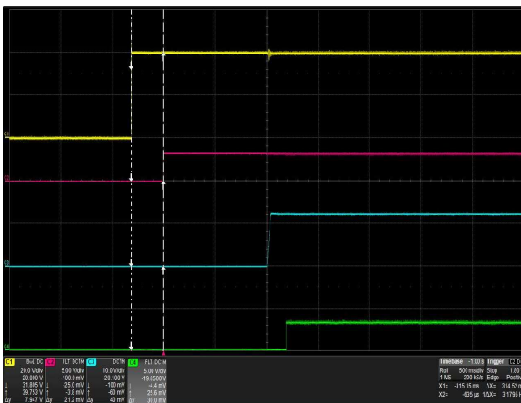
Figure 5: CSU2000ADC-3-100 VIN_GOOD Assert Characteristic Vin = -40Vdc Load: I_O = 10A I_{SB} = 1A Ch 1: V_{IN} Ch 2: VIN_GOOD Ch 3: V_O Ch 4: PWOK
