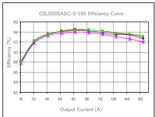
Figure 12: CSU2000ADC-3-100 Efficiency Curve @ 25°C Loading: I O,max = 10% increment to I O,max
