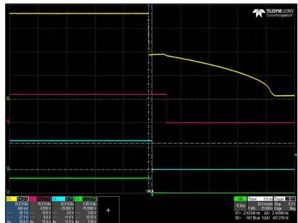
Figure 4: CSU2000ADC-3-100 Hold-Up Time Vin = -72Vdc Load: I_O = 163.9A I_{SB} = 3.5A Ch 1: V_{IN} Ch 2: V_{SB} Ch 3: V_O Ch 4: PWOK
