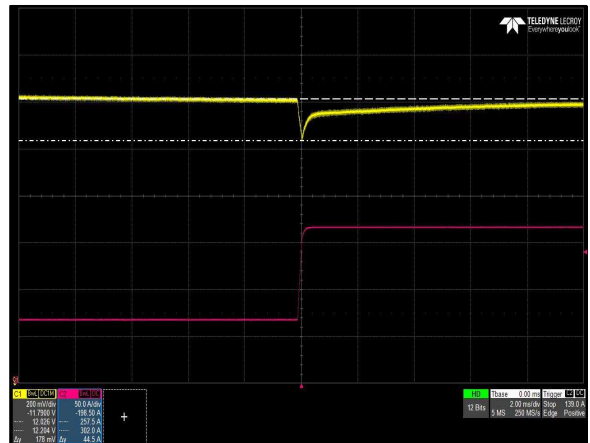
Figure 10: CSU2000ADC-3-100 Transient Response - V O Deviation 40% to 100% load change, 0.5A/μs slew rate, Vin = -48Vdc Ch 1: V O Ch 2: I O
