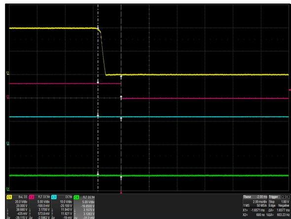
Figure 6: CSU2000ADC-3-100 VIN_GOOD De-assert Characteristic Vin = -40Vdc Load: I_O = 10A I_{SB} = 1A Ch 1: V_{IN} Ch 2: VIN_GOOD Ch 3: V_O Ch 4: PWOK
