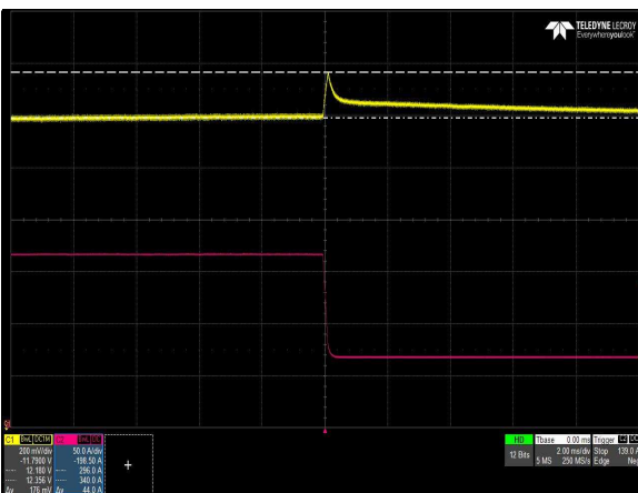
Figure 11: CSU2000ADC-3-100 Transient Response - V O Deviation 100% to 40% load change, 0.5A/μs slew rate, Vin = -48Vdc Ch 1: V O Ch 2: I O
