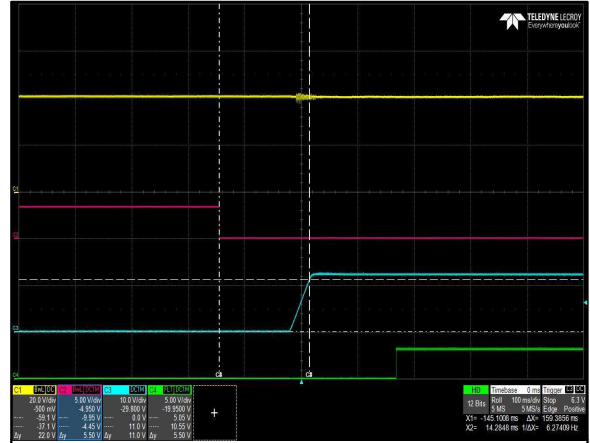
Figure 2: CSU2000ADC-3-100 Turn-On Delay via PSON Vin = -40Vdc Load: I_O = 163.9A I_{SB} = 3.5A Ch 1: V_{IN} Ch 2: PSON Ch 3: V_O Ch 4: PWOK
