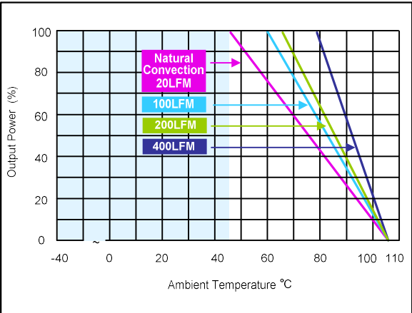
Figure 61: AEE10A36-L Derating Curves (without heatsink) Vin = 48Vdc Load: Io = 0 to 10A
