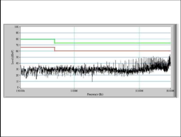
Figure 45: AEE02H18-L Conduction Emission of EN550122 Class A Vin = 24Vdc Load: Io = 2.08A
