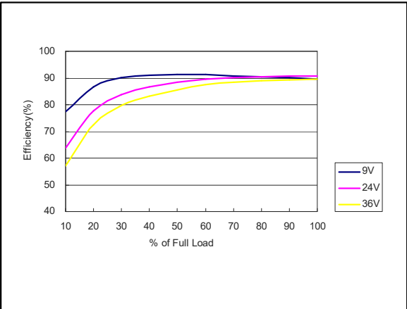
Figure 1: AEE10F18-L Efficiency Versus Output Current Curve Vin = 9 to 36Vdc Load: Io = 0 to 10A
