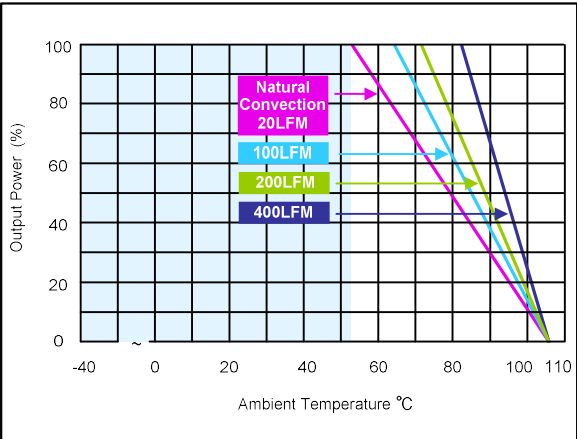
Figure 34: AEE03C18-L Derating Curves (without heatsink) Vin = 24Vdc Load: Io = 0 to 3.33A
