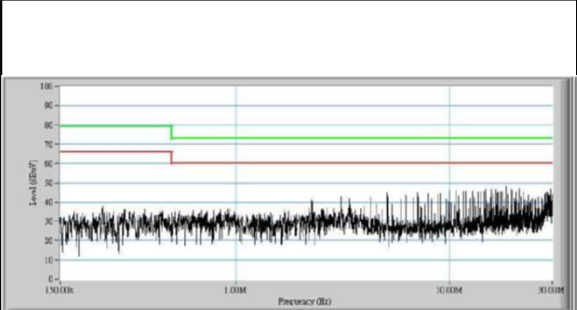
Figure 9: AEE10F18-L Conduction Emission of EN550122 Class A Vin = 24Vdc Load: Io = 10A
