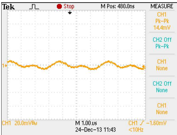
Figure 12: AEE10A18-L Ripple and Noise Measurement Vin = 24Vdc Load: Io = 10A Ch 1: Vo
