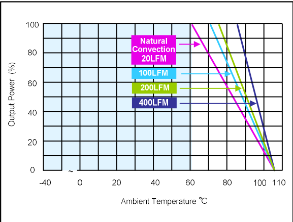
Figure 7: AEE10F18-L Derating Curves (without heatsink) Vin = 24Vdc Load: Io = 0 to 10A
