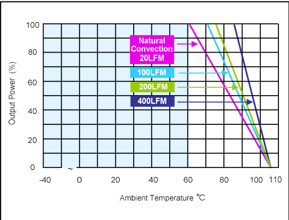
Figure 52: AEE10F36-L Derating Curves (without heatsink) Vin = 24Vdc Load: Io = 0 to 10A
