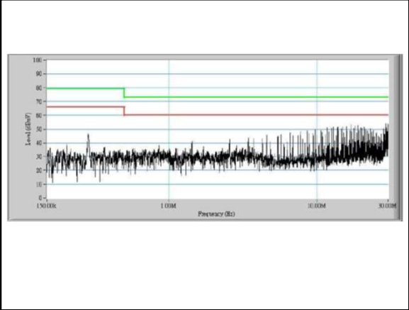
Figure 27: AEE04B18-L Conduction Emission of EN550122 Class A Vin = 24Vdc Load: Io = 4.17A
