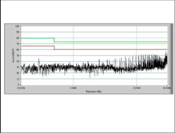
Figure 36: AEE03C18-L Conduction Emission of EN550122 Class A Vin = 24Vdc Load: Io = 3.33A
