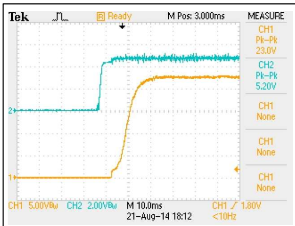
Figure 41: AEE02H18-L Output Voltage Startup Characteristic by On/Off Vin = 24Vdc Load: Io = 2.08A Ch 1: Vo Ch 2: Remote On/Off
