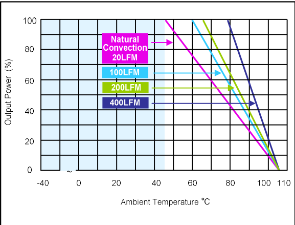
Figure 16: AEE10A18-L Derating Curves (without heatsink) Vin = 24Vdc Load: Io = 0 to 10A
