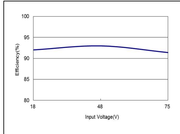
Figure 65: AEE04B36-L Efficiency Versus Input Voltage Curve Vin = 18 to 75Vdc Load: Io = 4.17A
