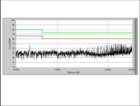
Figure 18: AEE10A18-L Conduction Emission of EN550122 Class A Vin = 24Vdc Load: Io = 10A
