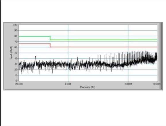
Figure 90: AEE02H36-L Conduction Emission of EN550122 Class A Vin = 48Vdc Load: Io = 2.08A
