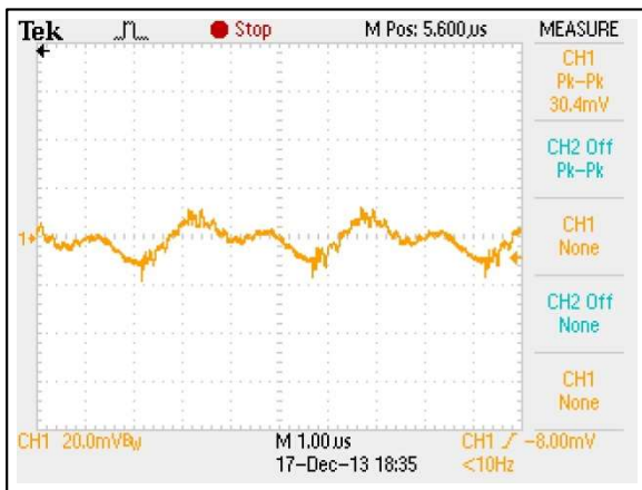
Figure 75: AEE03C36-L Ripple and Noise Measurement Vin = 48Vdc Load: Io = 3.33A Ch 1: Vo
