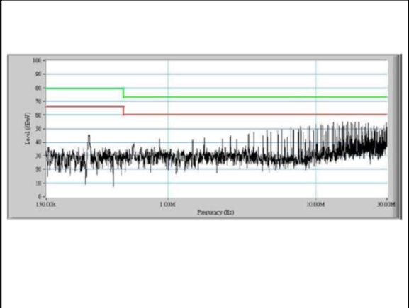
Figure 72: AEE04B36-L Conduction Emission of EN550122 Class A Vin = 48Vdc Load: Io = 4.17A
