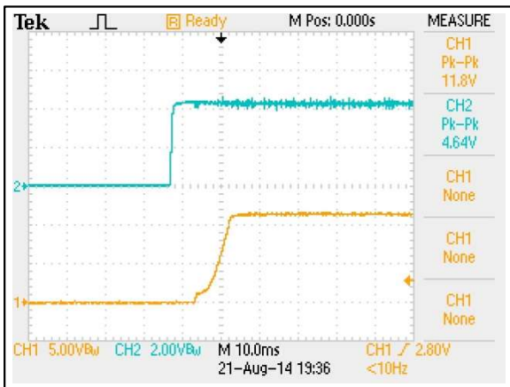
Figure 23: AEE04B18-L Output Voltage Startup Characteristic by On/Off Vin = 24Vdc Load: Io = 4.17A Ch 1: Vo Ch 2: Remote On/Off
