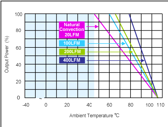
Figure 62: AEE10A36-L Derating Curves (with heatsink) Vin = 48Vdc Load: Io = 0 to 10A
