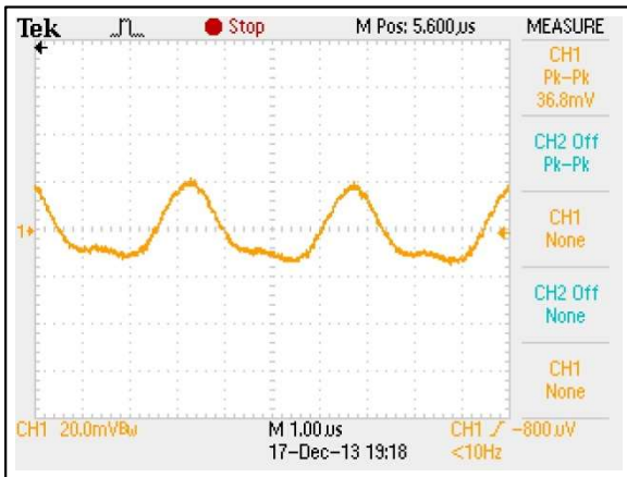
Figure 66: AEE04B36-L Ripple and Noise Measurement Vin = 48Vdc Load: Io = 4.17A Ch 1: Vo
