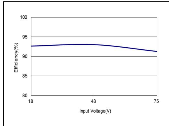
Figure 74: AEE03C36-L Efficiency Versus Input Voltage Curve Vin = 18 to 75Vdc Load: Io = 3.33A
