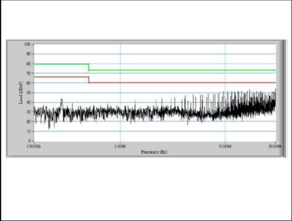
Figure 54: AEE10F36-L Conduction Emission of EN550122 Class A Vin = 24Vdc Load: Io = 10A
