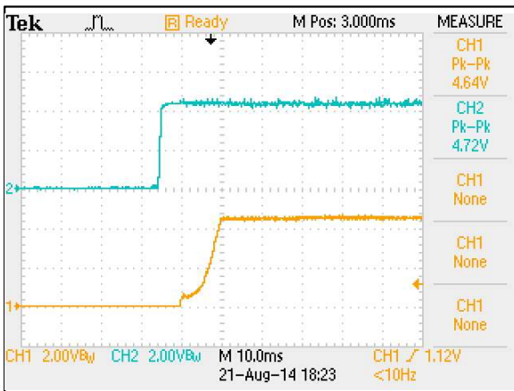
Figure 14: AEE10A18-L Output Voltage Startup Characteristic by On/Off Vin = 24Vdc Load: Io = 10A Ch 1: Vo Ch 2: Remote On/Off
