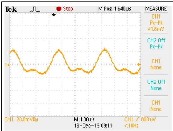
Figure 21: AEE04B18-L Ripple and Noise Measurement Vin = 24Vdc Load: Io = 4.17A Ch 1: Vo
