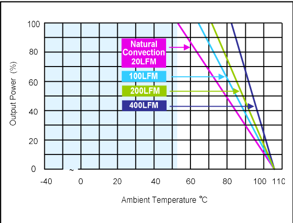
Figure 25: AEE04B18-L Derating Curves (without heatsink) Vin = 24Vdc Load: Io = 0 to 4.17A
