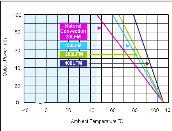
Figure 43: AEE02H18-L Derating Curves (without heatsink) Vin = 24Vdc Load: Io = 0 to 2.08A
