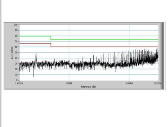
Figure 81: AEE03C36-L Conduction Emission of EN550122 Class A Vin = 48Vdc Load: Io = 3.33A
