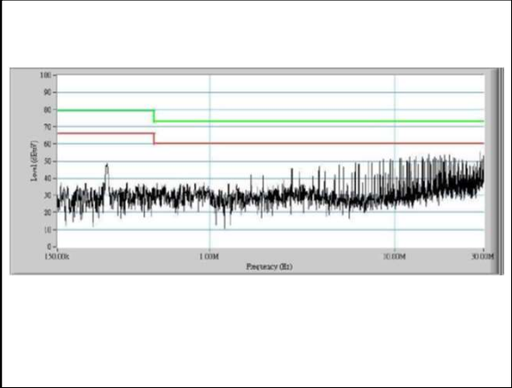
Figure 63: AEE10A36-L Conduction Emission of EN550122 Class A Vin = 48Vdc Load: Io = 10A
