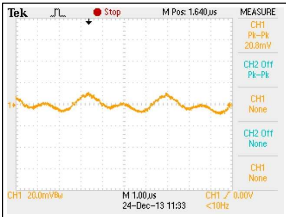
Figure 57: AEE10A36-L Ripple and Noise Measurement Vin = 48Vdc Load: Io = 10A Ch 1: Vo
