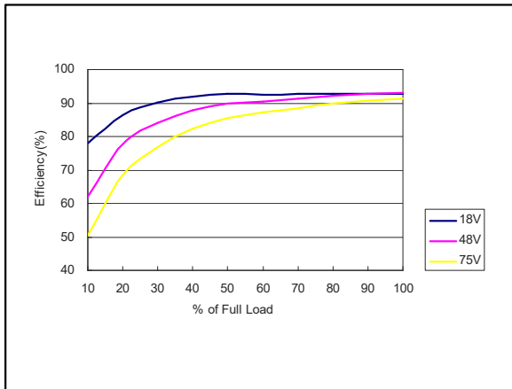
Figure 73: AEE03C36-L Efficiency Versus Output Current Curve Vin = 18 to 75Vdc Load: Io = 0 to 3.33A
