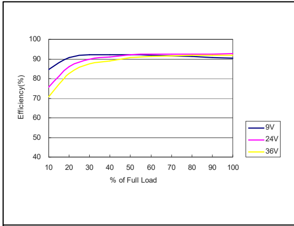
Figure 37: AEE02H18-L Efficiency Versus Output Current Curve Vin = 9 to 36Vdc Load: Io = 0 to 2.08A
