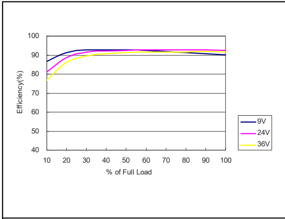
Figure 10: AEE10A18-L Efficiency Versus Output Current Curve Vin = 9 to 36Vdc Load: Io = 0 to 10A
