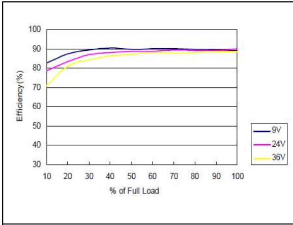
Figure 19: AEE04B18-L Efficiency Versus Output Current Curve Vin = 9 to 36Vdc Load: Io = 0 to 4.17A
