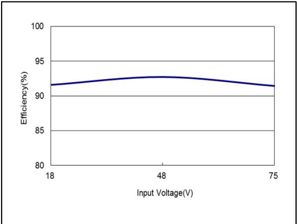
Figure 83: AEE02H36-L Efficiency Versus Input Voltage Curve Vin = 18 to 75Vdc Load: Io = 2.08A
