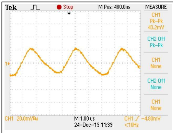
Figure 39: AEE02H18-L Ripple and Noise Measurement Vin = 24Vdc Load: Io = 2.08A Ch 1: Vo
