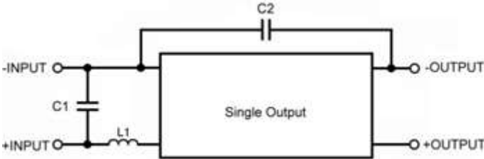
Recommended circuit to comply EN55022 Class A limits
