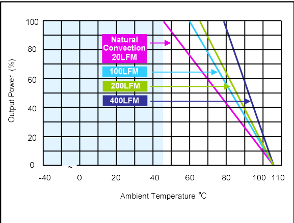
Figure 88: AEE02H36-L Derating Curves (without heatsink) Vin = 48Vdc Load: Io = 0 to 2.08A
