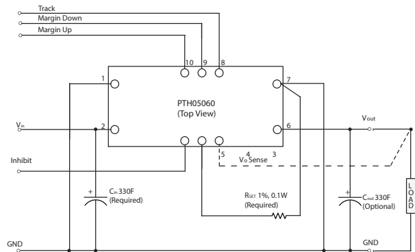
Figure 4 - Standard Application
