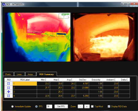
View of the melt tank with LumaSpec RT software
