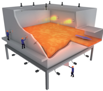
Obtaining reliable temperature measurement in the melting tank
