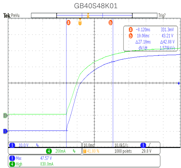
Figure 26: Turn-on rise time at 264Vac - 0.83A load
