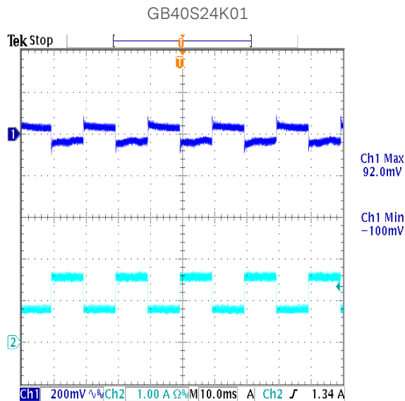
Figure 56: Transient Response at 230Vac, 50%-100% step load CH1:Vout CH2: Load Current
