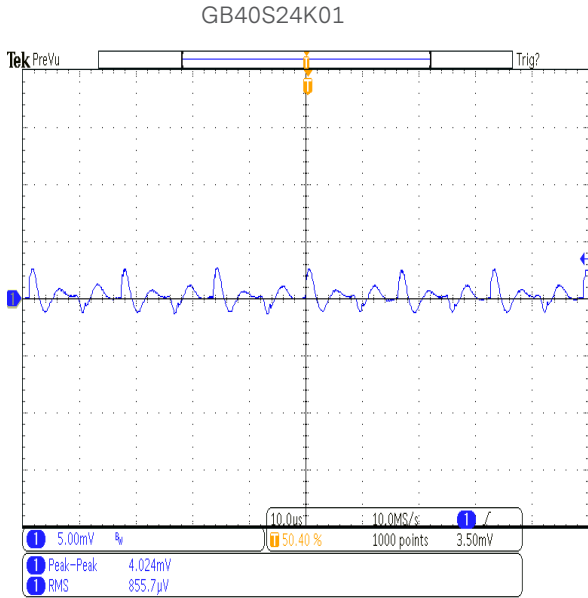
Figure 63: Common Mode Current at 115Vac Current Probe:1mA/mV
