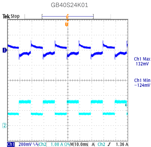
Figure 55: Transient Response at 115Vac, 50%-100% step load CH1: Vout CH2: Load Current
