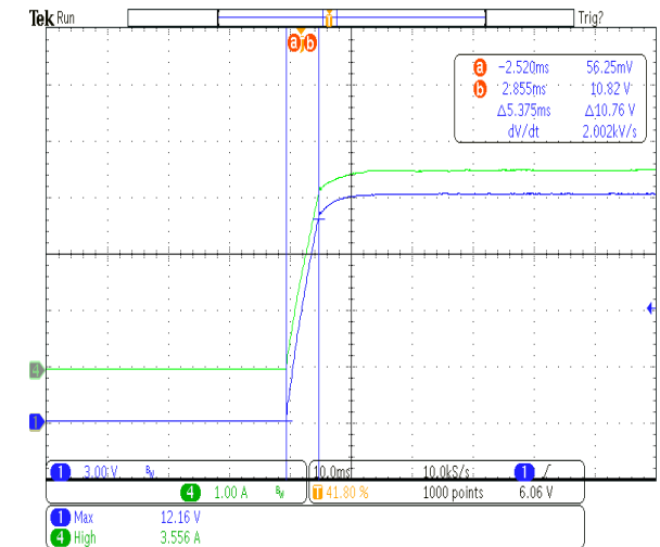
Figure 22: Turn-on rise time at 264Vac - 3.4A load
