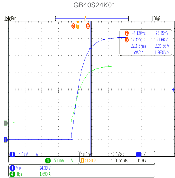
Figure 24: Turn-on rise time at 264Vac - 1.7A load
