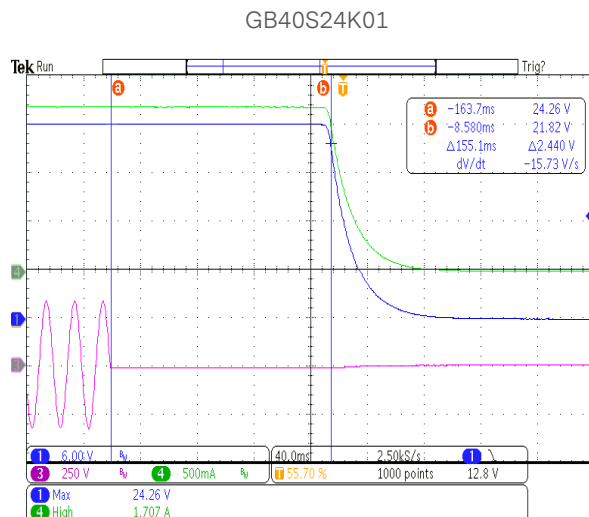
Figure 32: Hold-up time at 230Vac - 1.7A load
