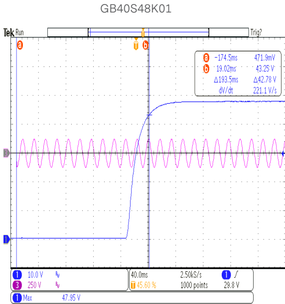
Figure 17: Turn-on delay at 90Vac - 0.83A load
