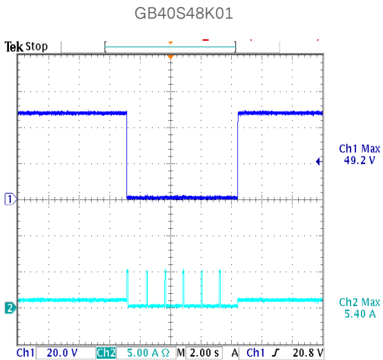
Figure 49: Output Over Load at 115Vac
