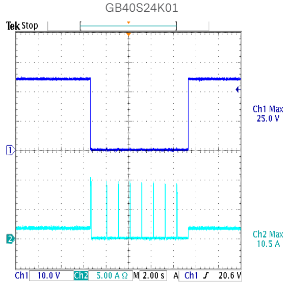
Figure 48: Output Over Load at 230Vac
