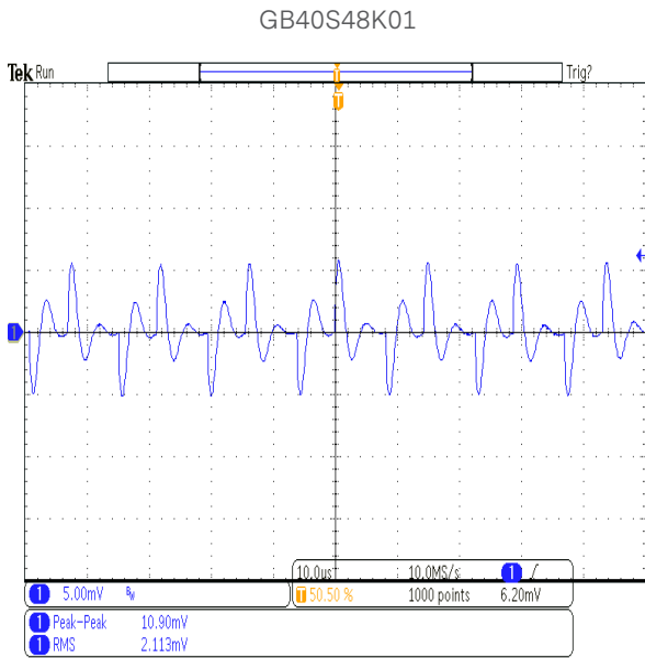
Figure 65: Common Mode Current at 115Vac Current Probe:1mA/mV
