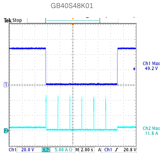
Figure 50: Output Over Load at 230Vac
