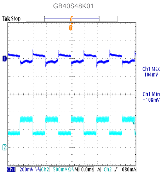
Figure 57: Transient Response at 115Vac, 50%-100% step load CH1: Vout CH2: Load Current
