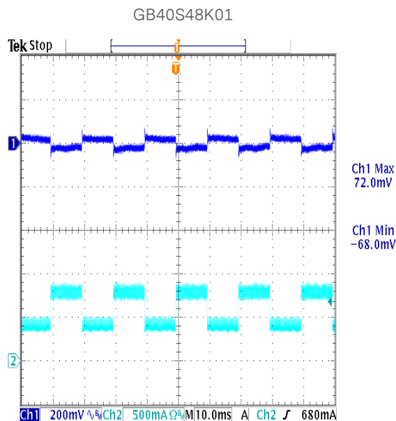
Figure 58: Transient Response at 230Vac, 50%-100% step load CH1:Vout CH2: Load Current
