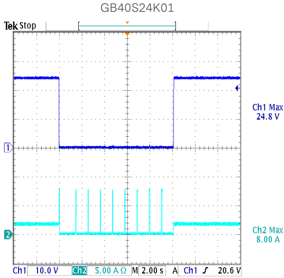
Figure 47: Output Over Load at 115Vac
