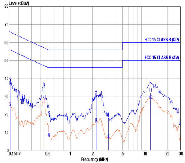
Figure 77: EN55032 CLASS B – 120V/60Hz 10% Load magin >10 dB Blue Plot: Quasi-Peak. Red Plot: Average.
