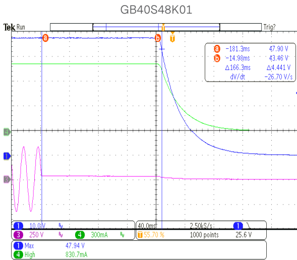
Figure 34: Turn-on rise time at 230Vac - 0.83A load
