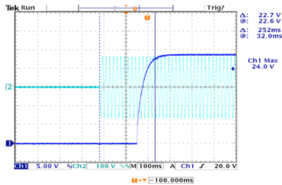
24V Turn-on delay, 115VAC
