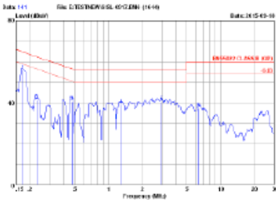
CISPR22 CLASS B QP 230V/50Hz 100% LOAD MARGIN: >9 dB
