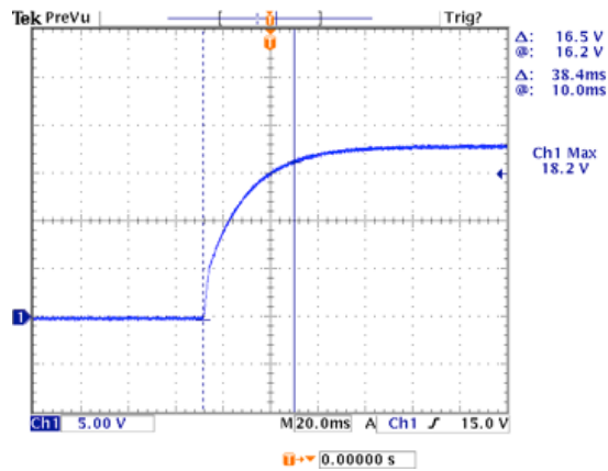
18V Rise Time
