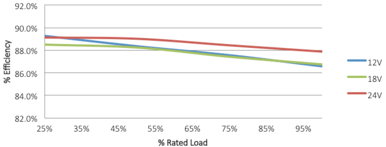
FIGURE 5: ME40 Series Efficiency @ 115VAC.
