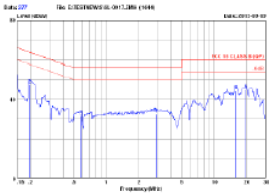
FCC15 CLASS B QP 120V/60Hz 100% LOAD MARGIN: >15 dB
