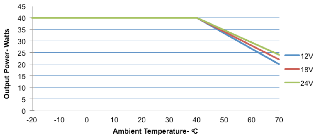
FIGURE 2: ME40 family derating curve.
